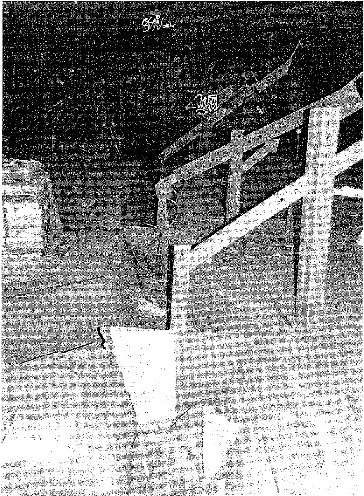
Photograph #16 CARRIE BLAST FURNACES NUMBER 6 AND 7 Allegheny County, PA Detail of iron runners and gates, furnace number 6 cast house. Photographers: Ron Baraff and Michael Bennett, June 23, 2000.
